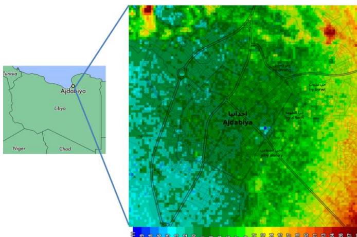
Figure 2: Location and topography Ajdabiya City ( https://elevation.city/ly/1wrdr ).
